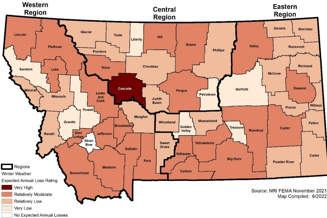
Figure 4-62 NRI Expected Annual Loss Rating from Winter Weather
