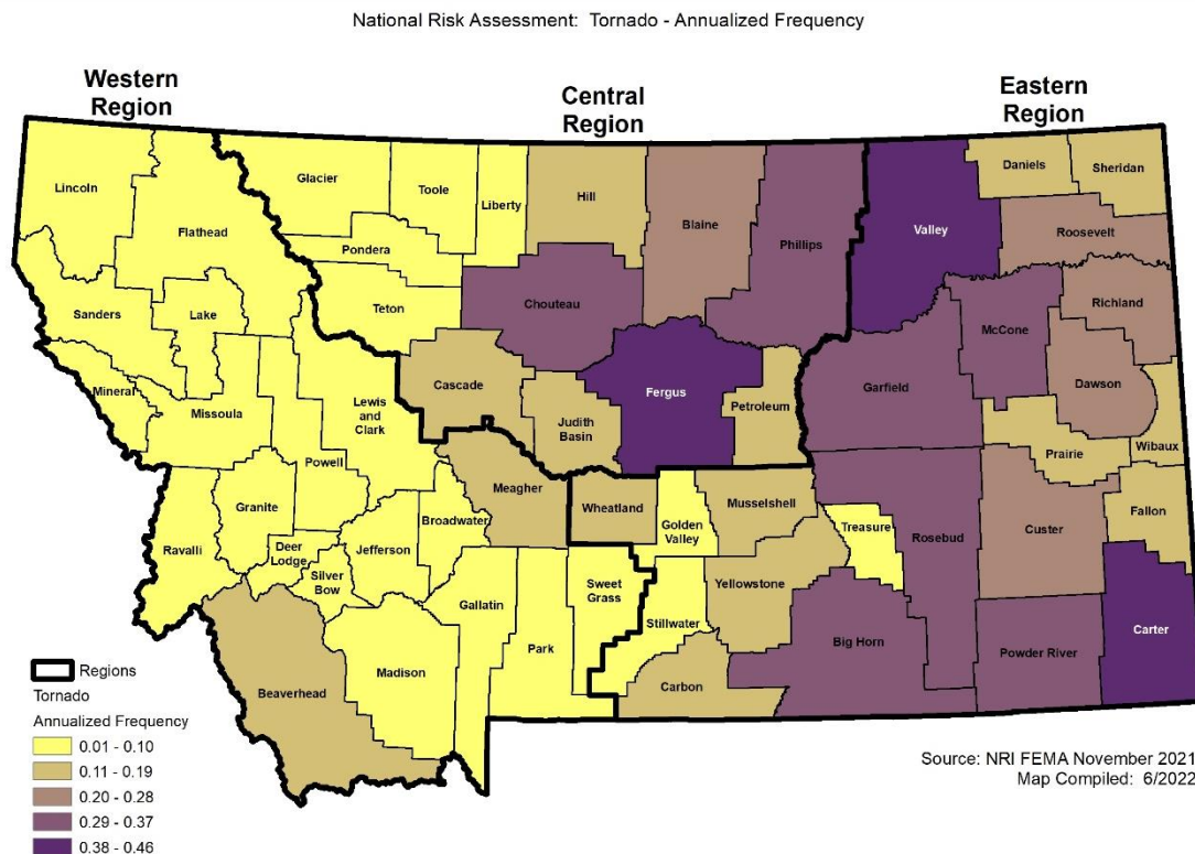
Figure 4-72 Annualized Frequency of Tornado Events by County
