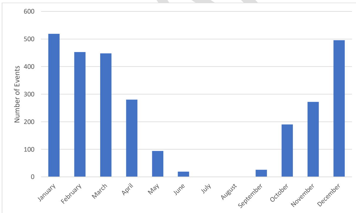
Figure 4-58 Monthly Trend of Winter Weather Events in the Eastern Region (1996-2022)
