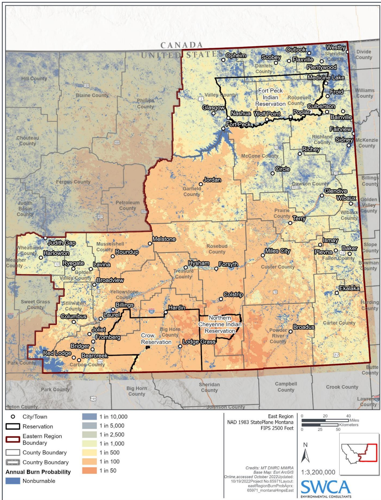
Figure 4-96 Eastern Montana Region Annual Burn Probability
