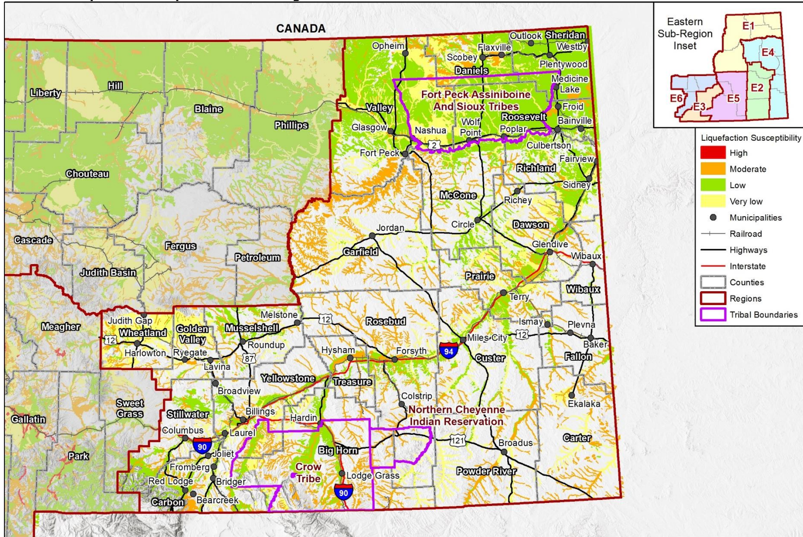
Figure 4-24 Liquefaction Map of the Eastern Region
