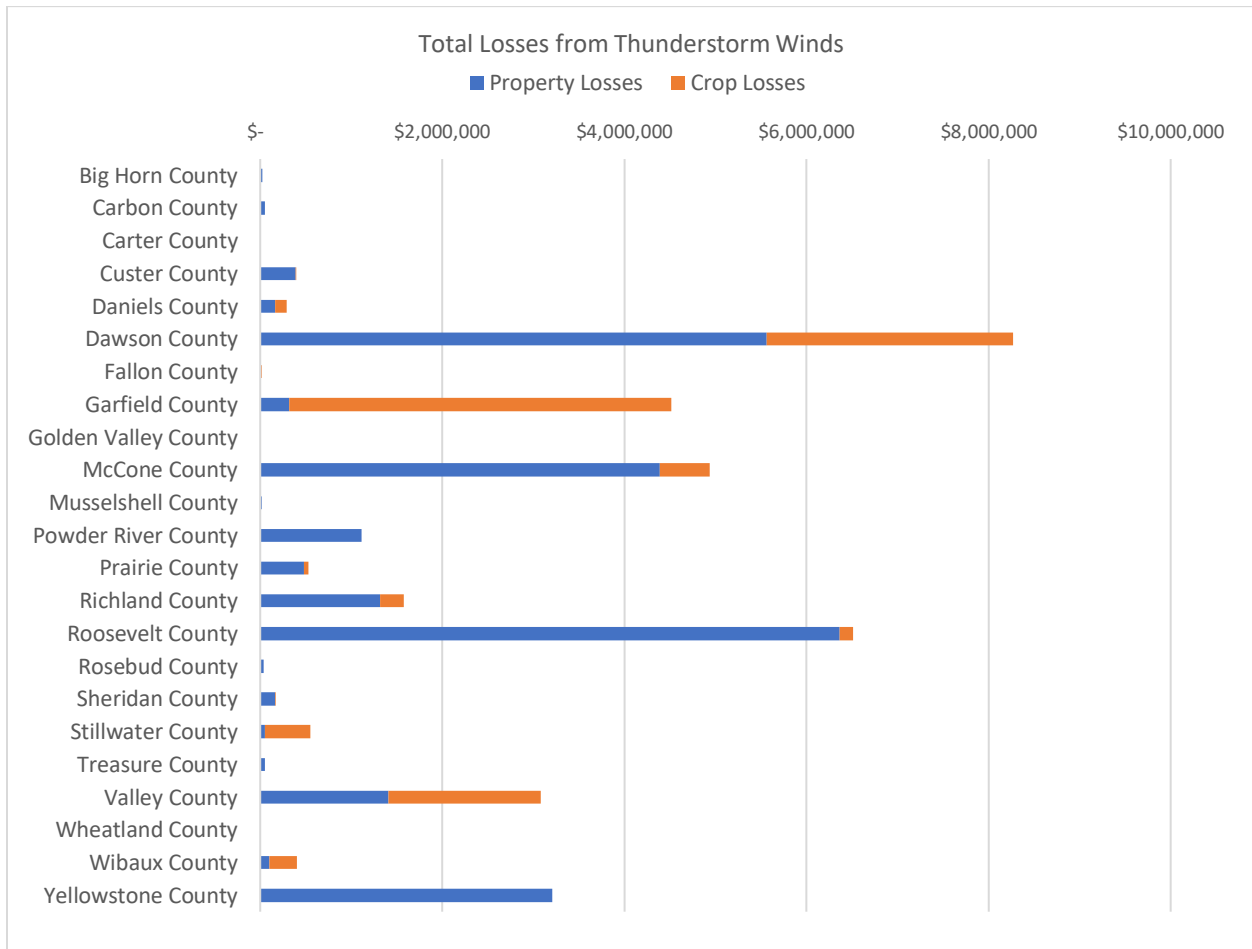
Figure 4-70 Total Losses from Thunderstorm Wind by County
