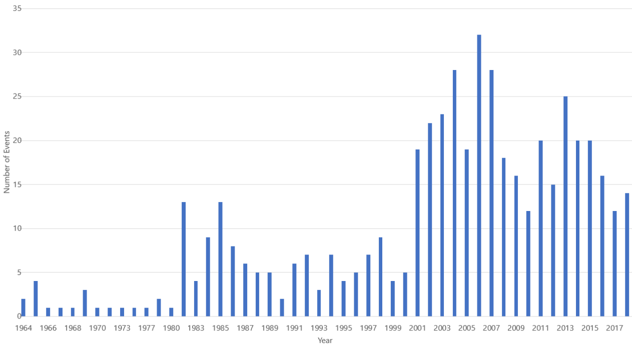
Figure 4-78 Annual Aircraft Incidents in the State of Montana
