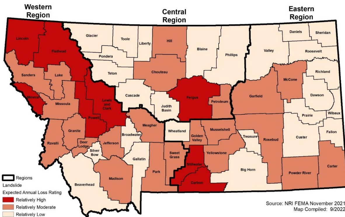
Figure 4-43 NRI Expected Annual Loss Rating Montana Eastern Region
