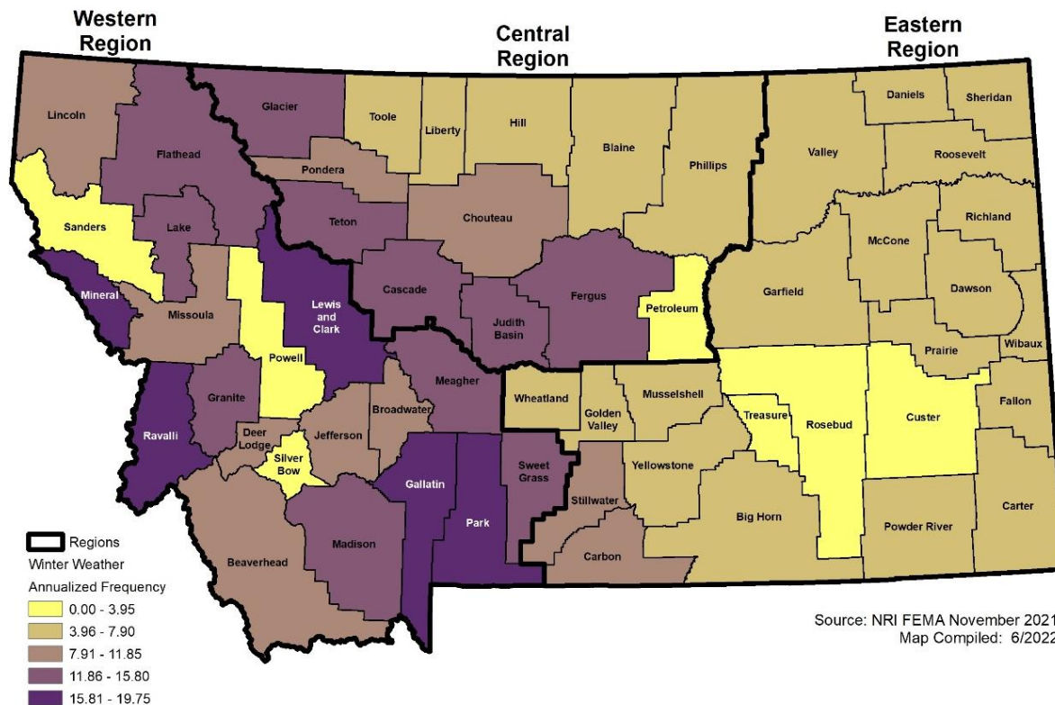
Figure 4-56 NRI Annualized Frequency of Winter Weather Events by County
