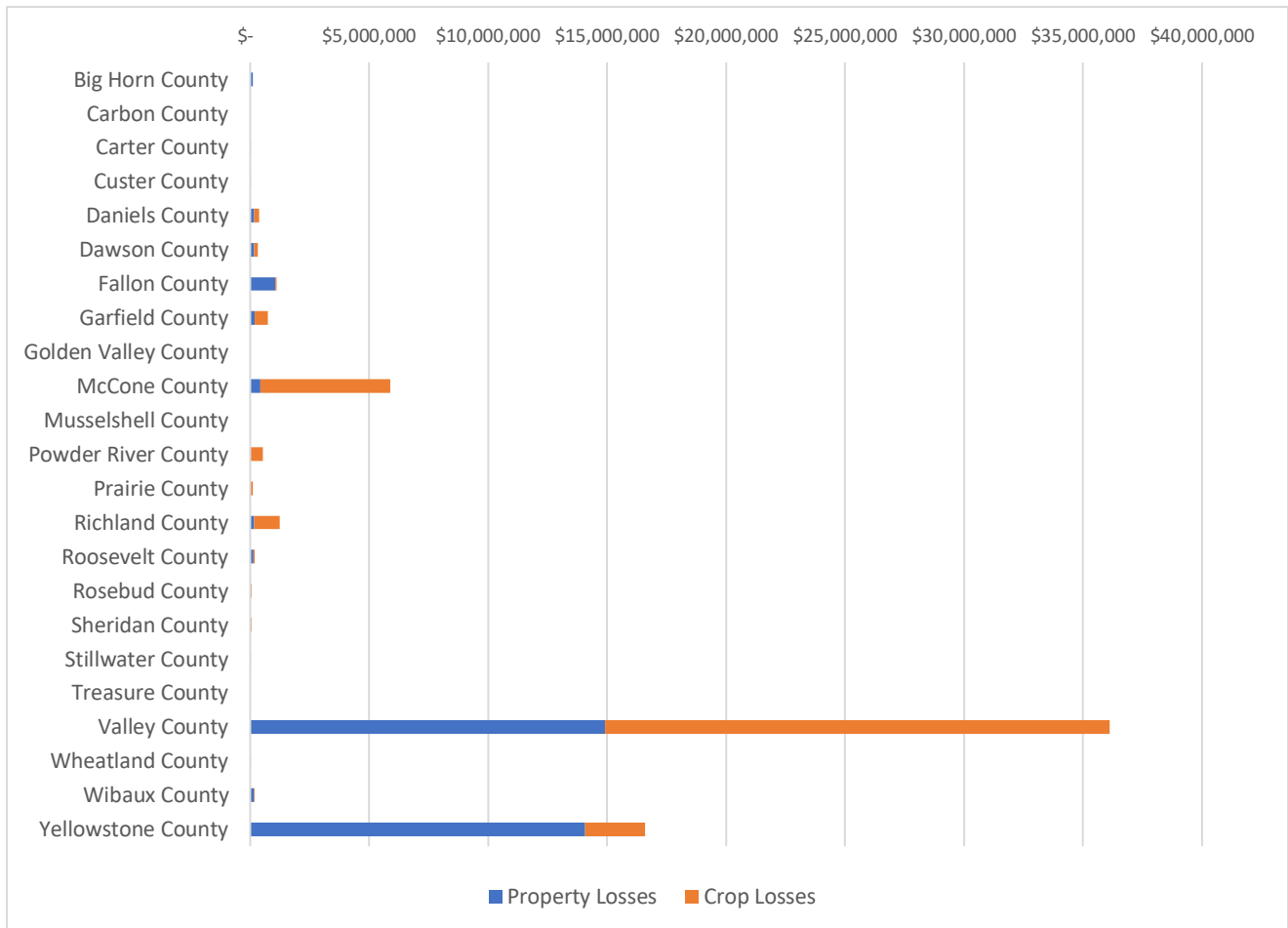
Figure 4-46 Summary of Severe Summer Weather Events by County in the Eastern Region
