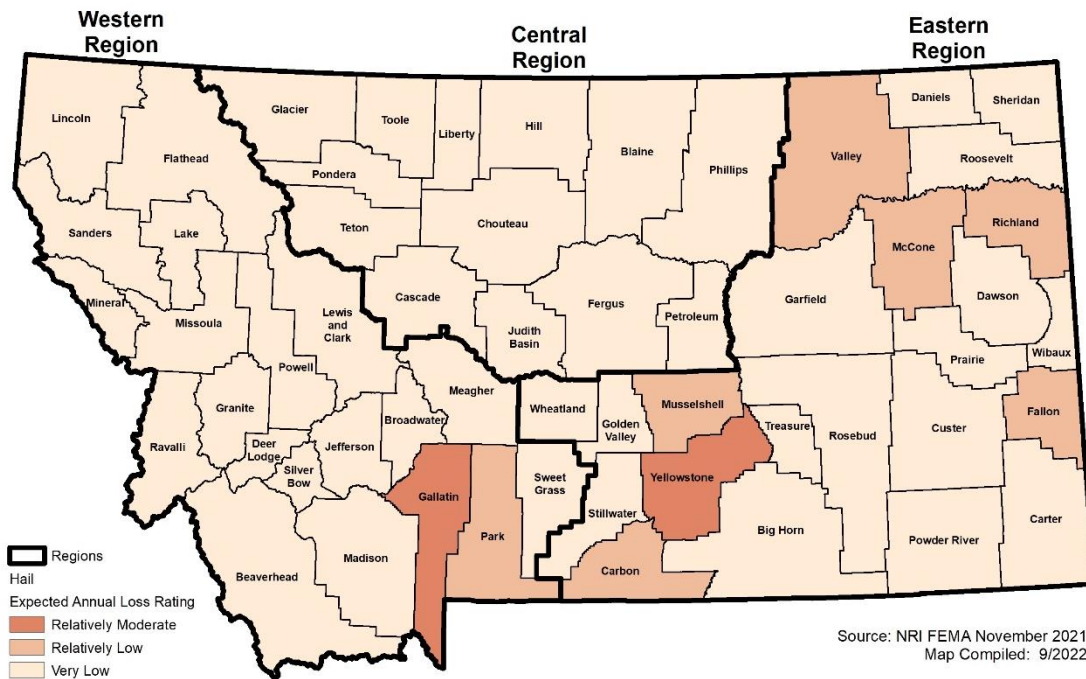
Figure 4-52 NRI Hail Expected Annual Loss Rating
