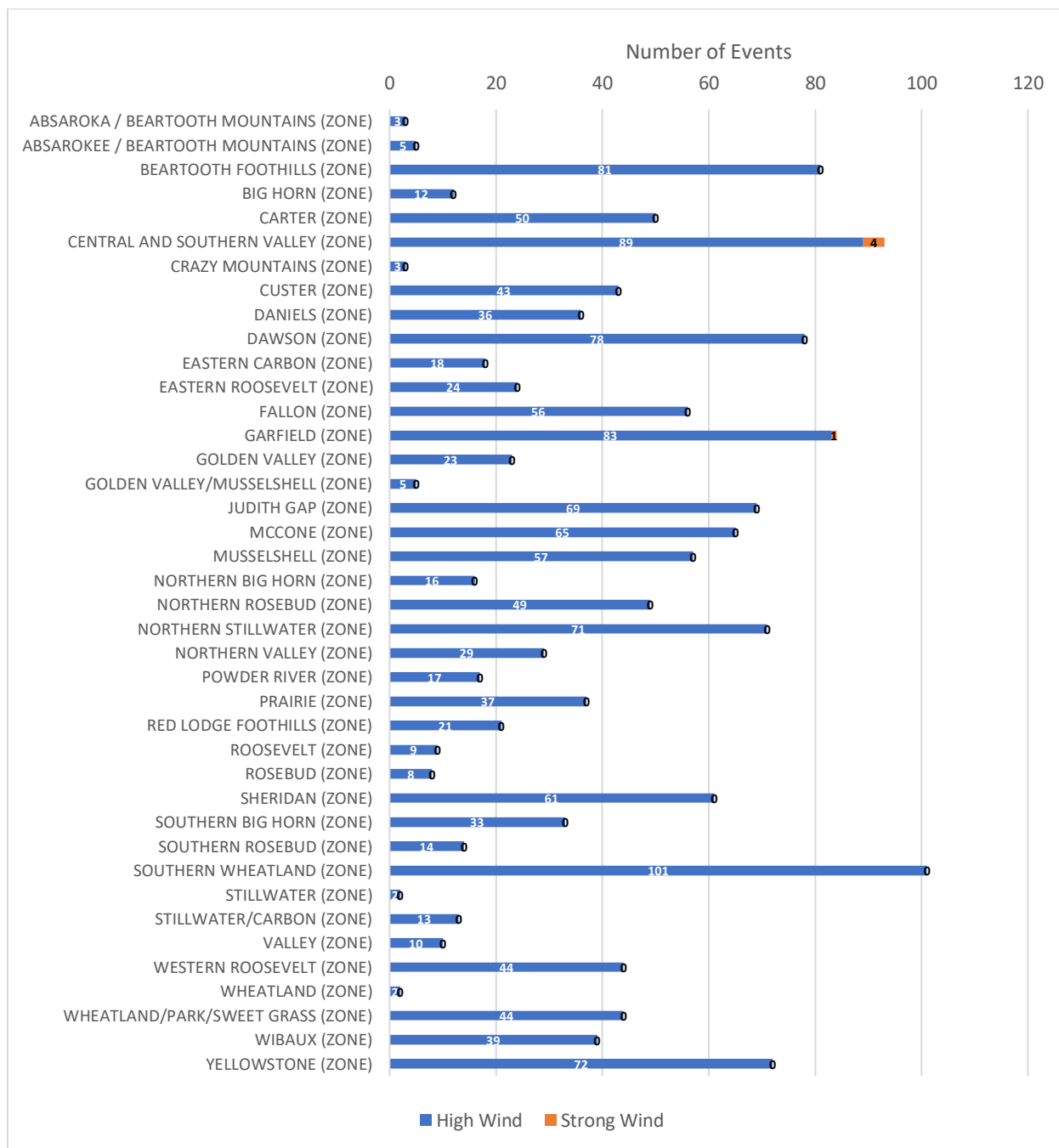
Figure 4-69 Total High Wind and Strong Wind Events by Zone (1996 to 2022)
