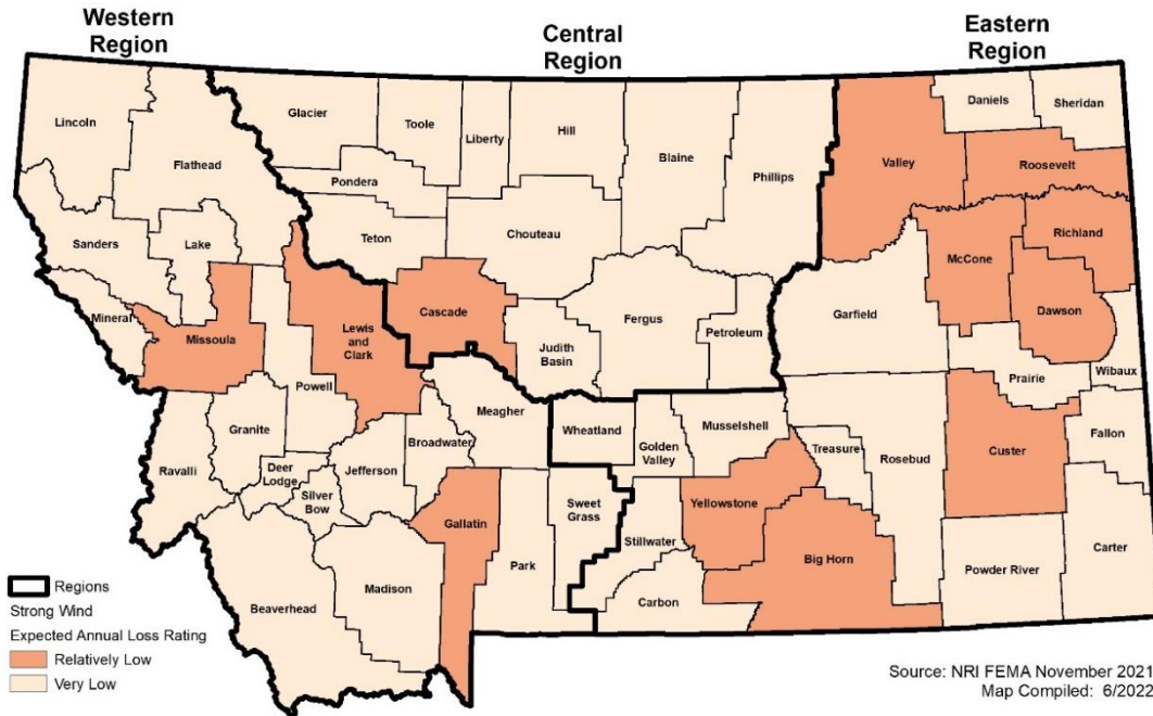
Figure 4-76 NRI Strong Wind Expected Annual Loss Rating
