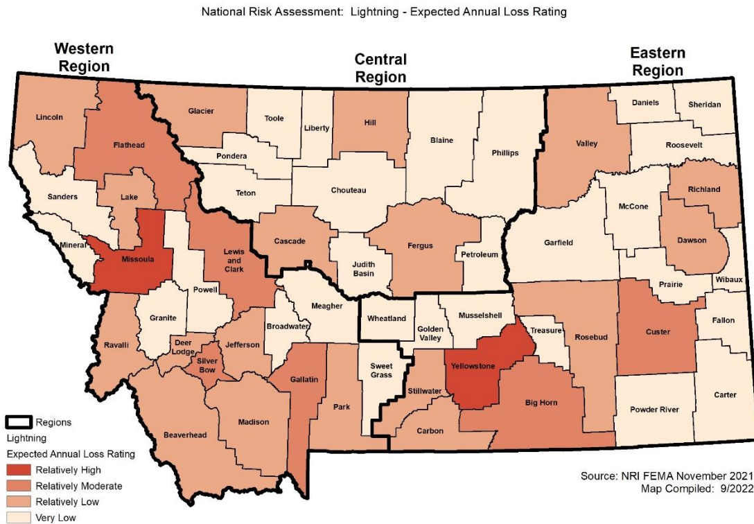
Figure 4-53 NRI Lightning Expected Annual Loss Rating
