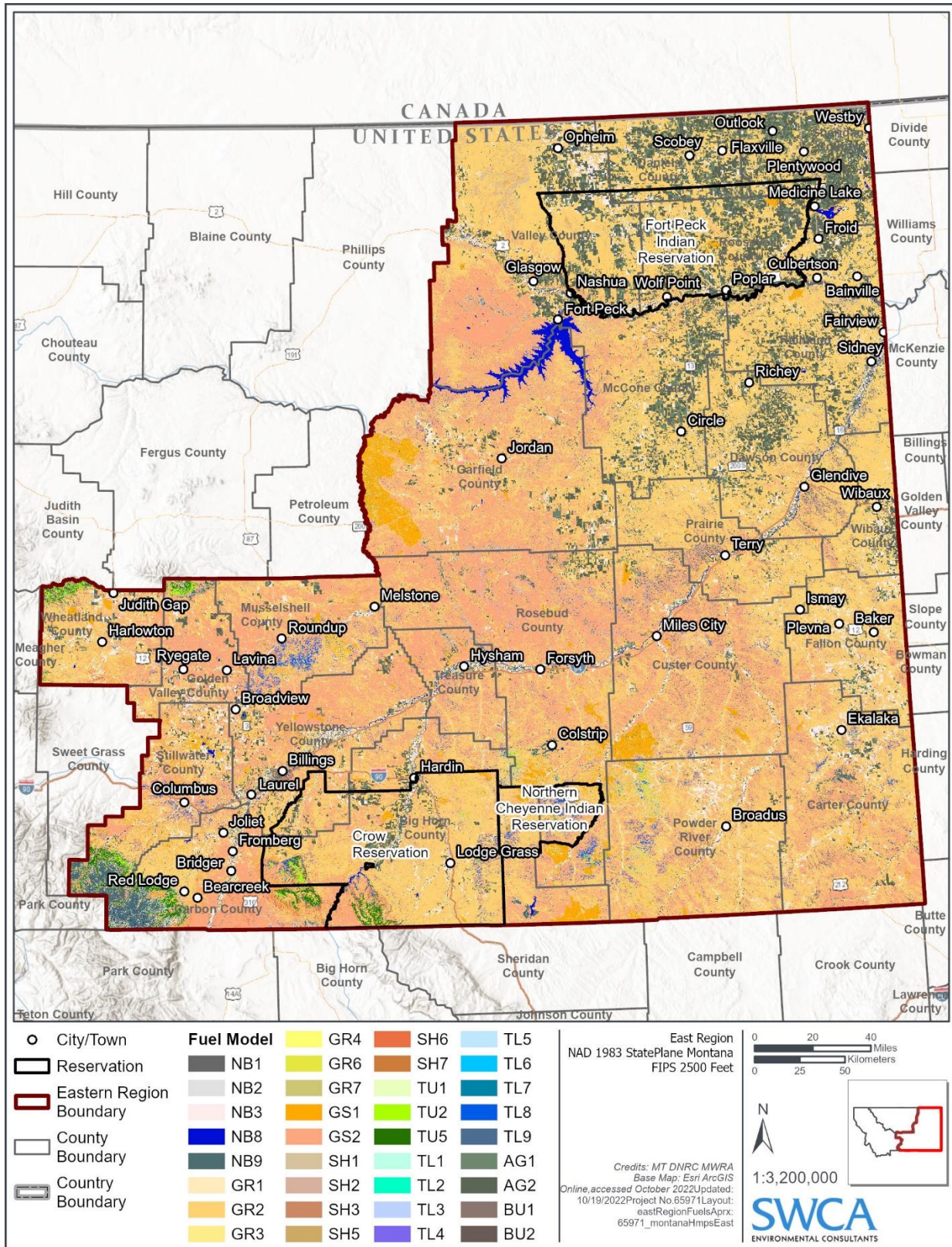
Figure 4-85 Wildfire Fuel Model of the Eastern Region
