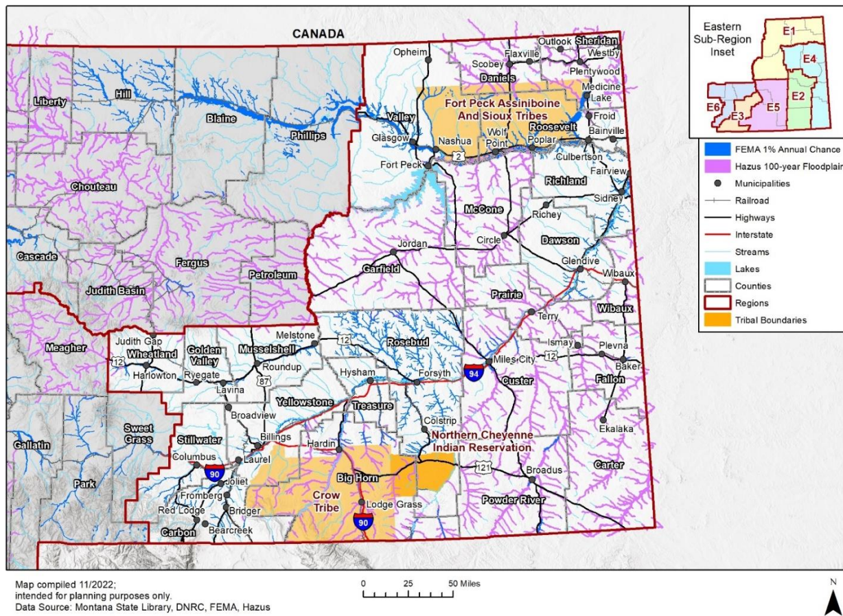
Figure 4-28 Eastern Region Flood Hazards (NFHL and Hazus)
