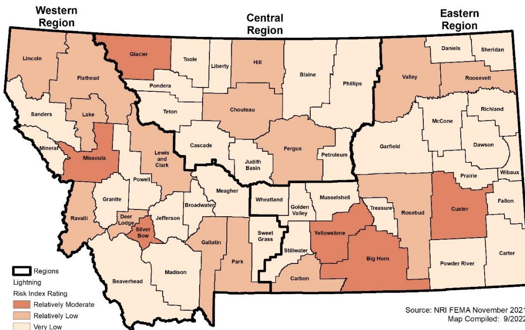
Figure 4-51 NRI Risk Index Rating for Lightning
