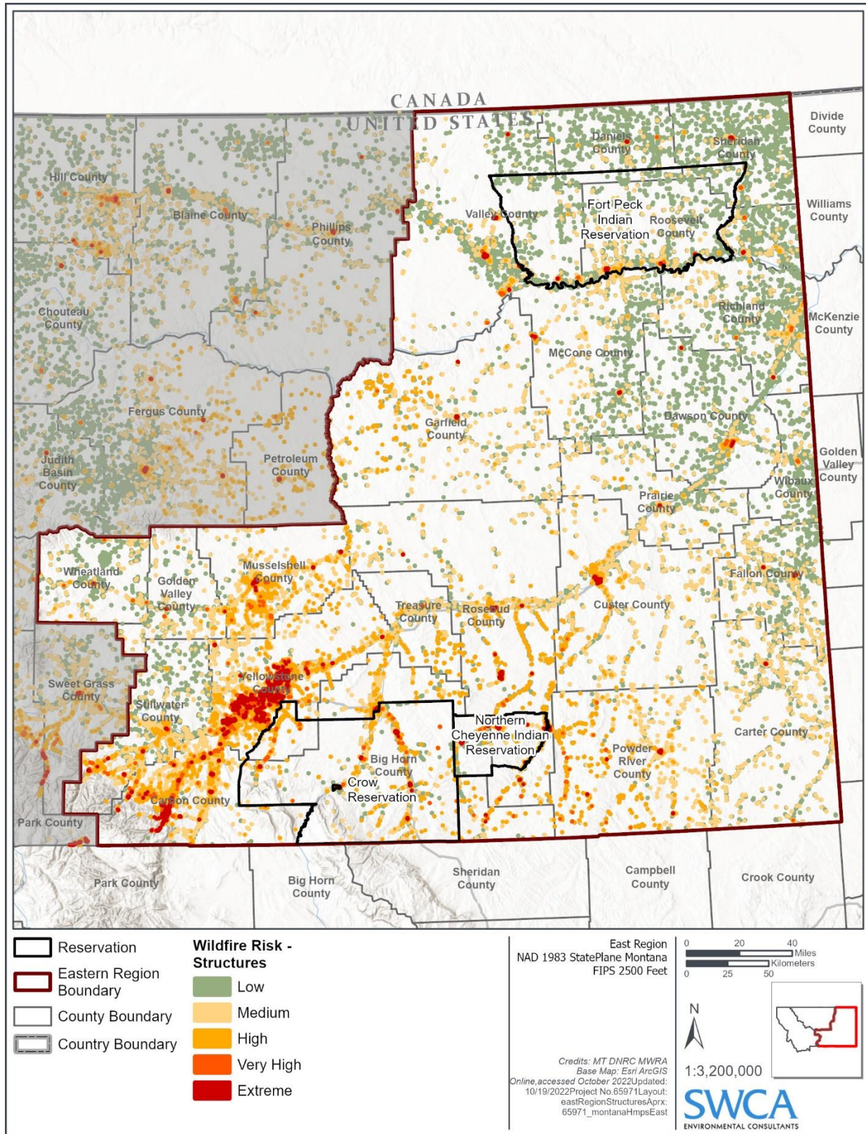
Figure 4-101 Wildfire Risk to Structures in the Eastern Region
