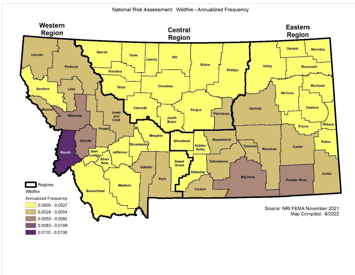
Figure 4-95 Annualized Frequency of Wildfire Events by County
