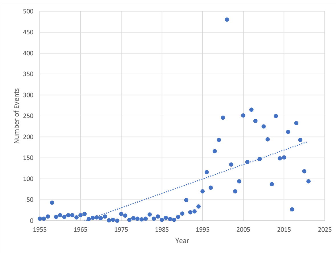
Figure 4-47 Hail Events by Year in the Eastern Region (1955-2021)
