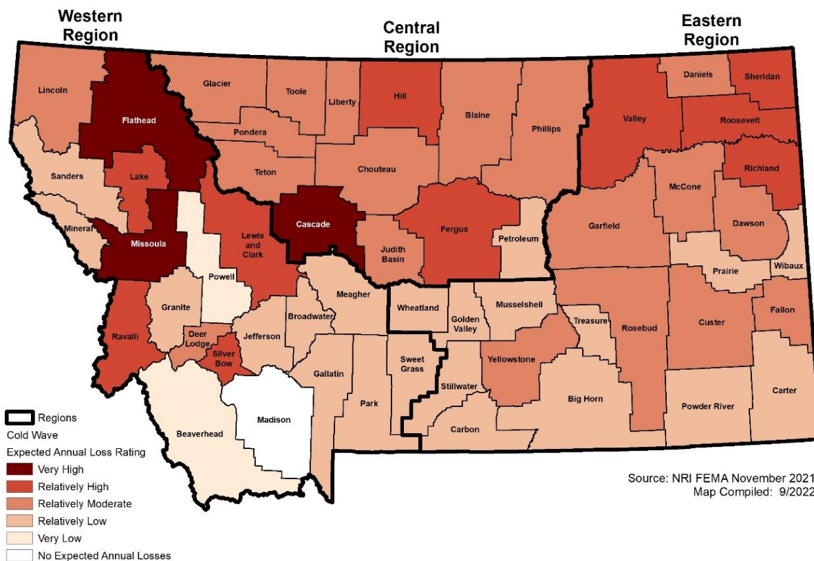
Figure 4-61 NRI Expected Annual Loss Rating from Cold Waves
