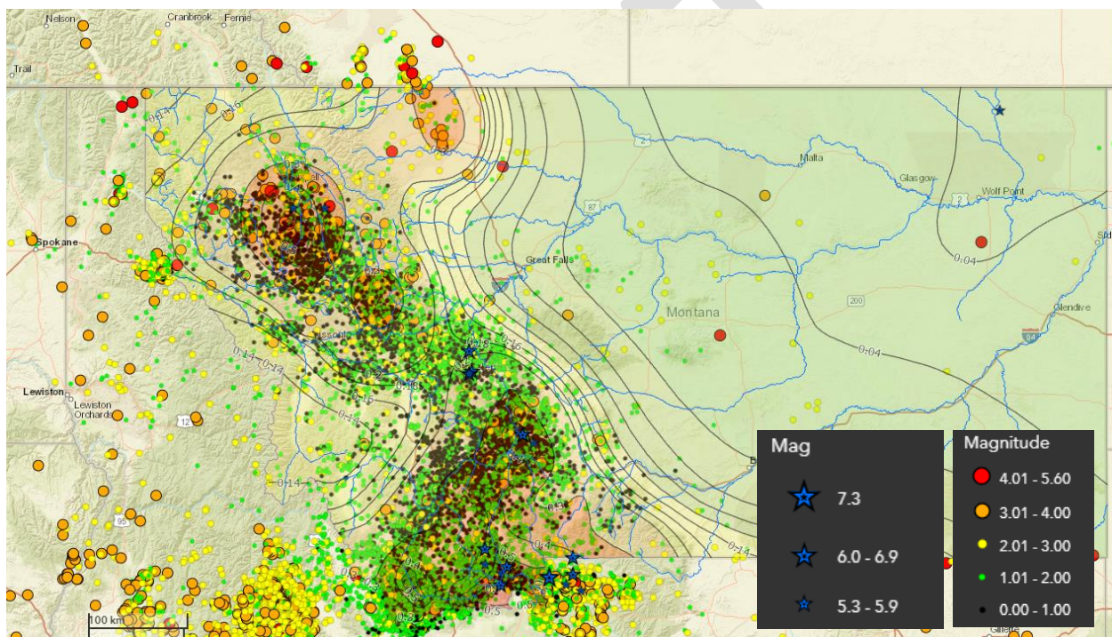
Figure 4-25 Statewide Map of Earthquake Epicenters, 1982-2022
