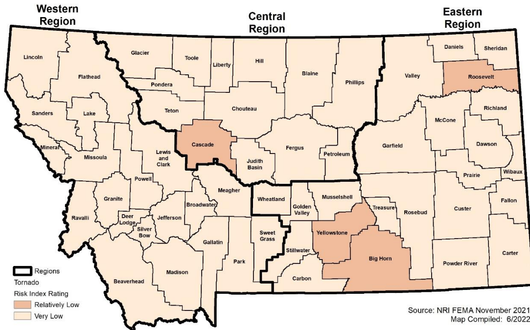
Figure 4-75 NRI Risk Index Rating for Tornadoes
