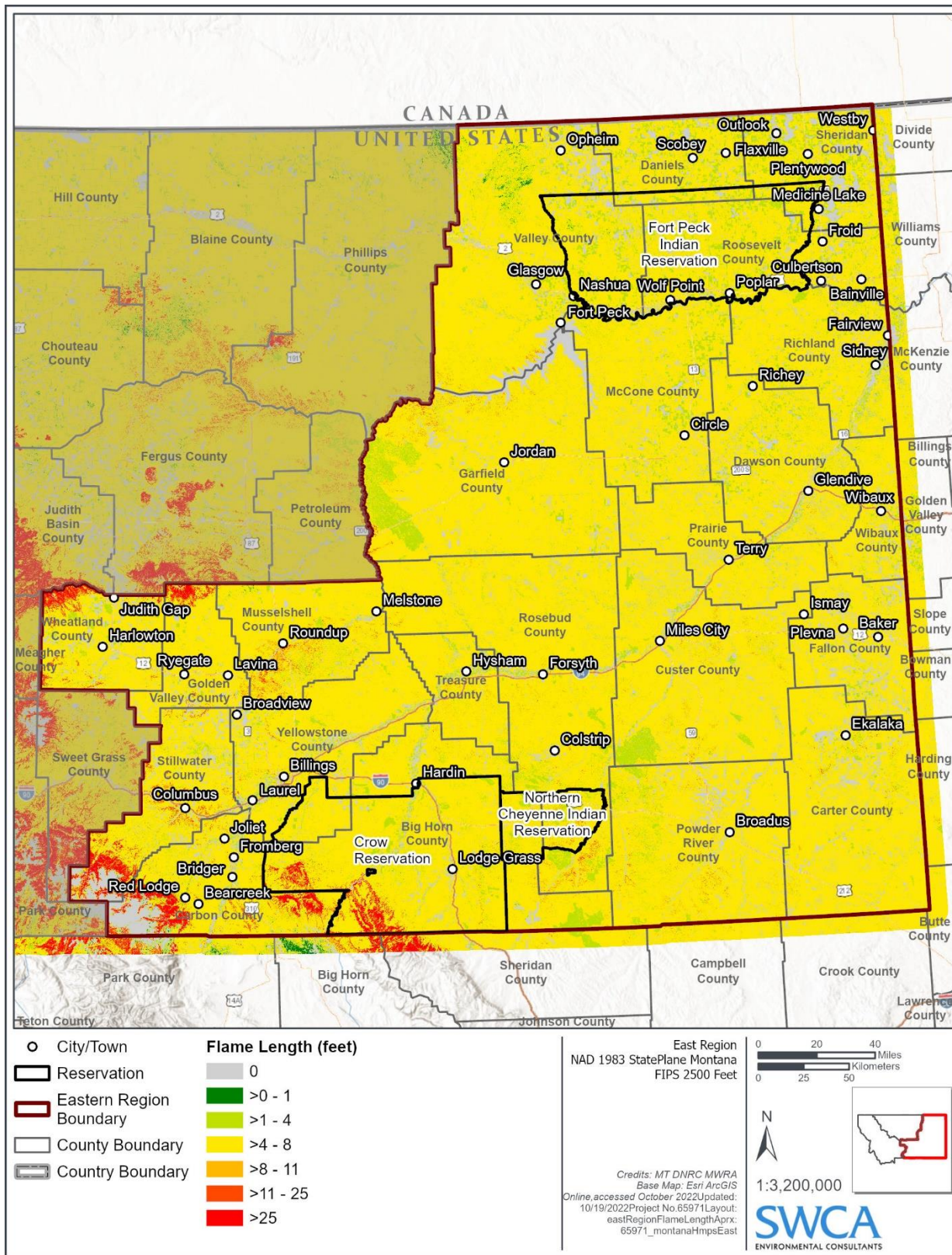
Figure 4-98 Eastern Montana Region Estimated Flame Length
