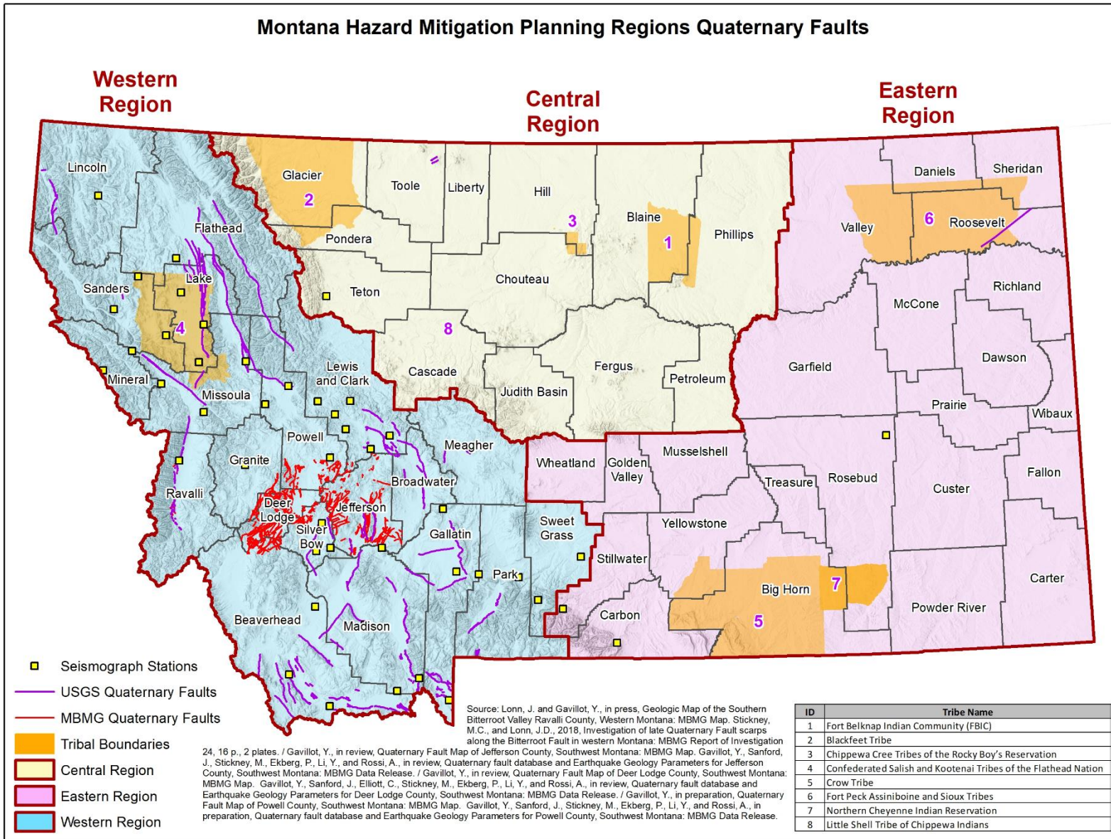
Figure 4-23 Fault Map of Montana
