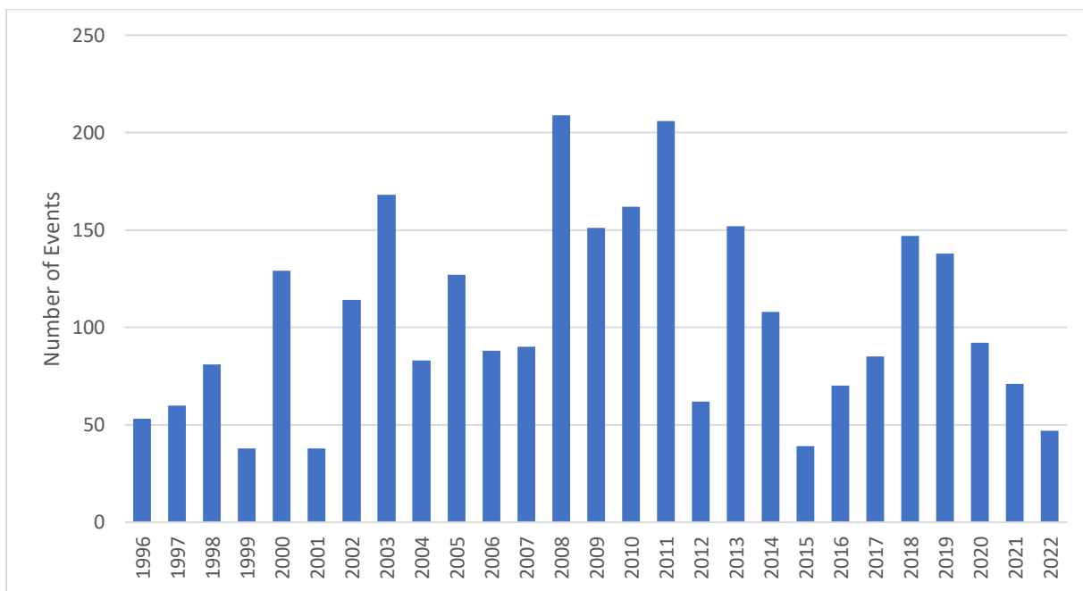
Figure 4-57 Yearly Trend of Winter Weather Events in the Eastern Region (1996-2022)
