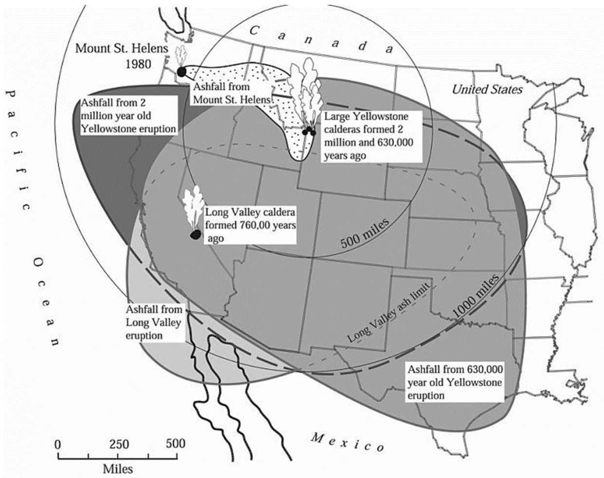
Figure 4-84 Areas of the United States once covered by volcanic ash from major eruptions
