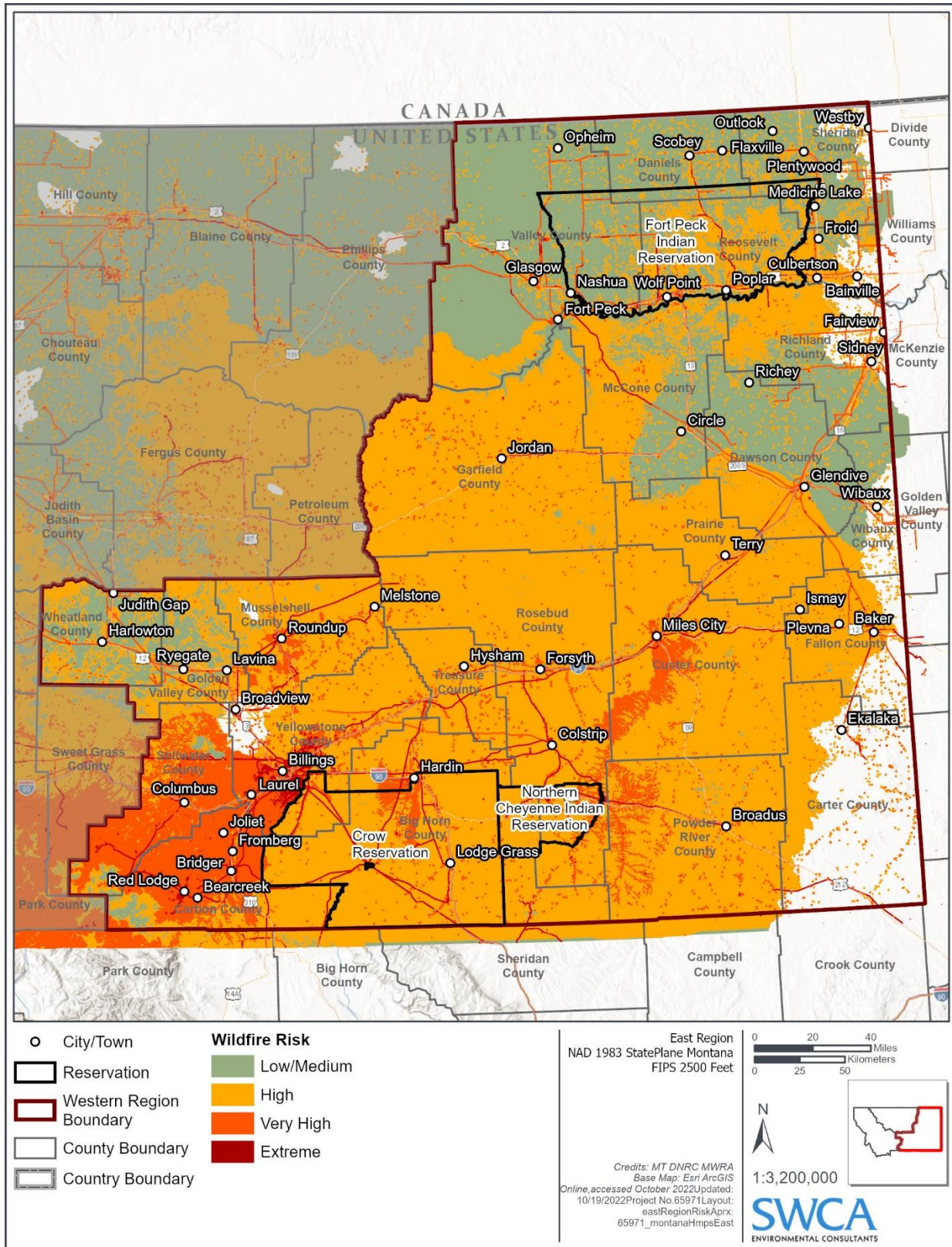
Figure 4-99 Eastern Region Wildfire Risk Summary as Determined by eNVC
