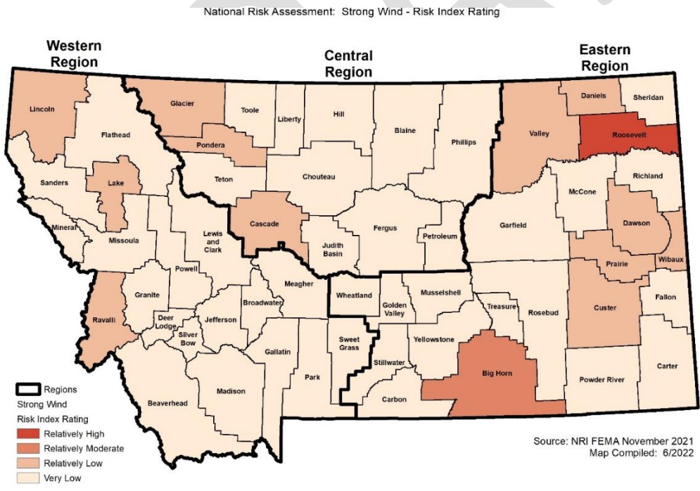
Figure 4-74 NRI Risk Index Rating for Strong Wind
