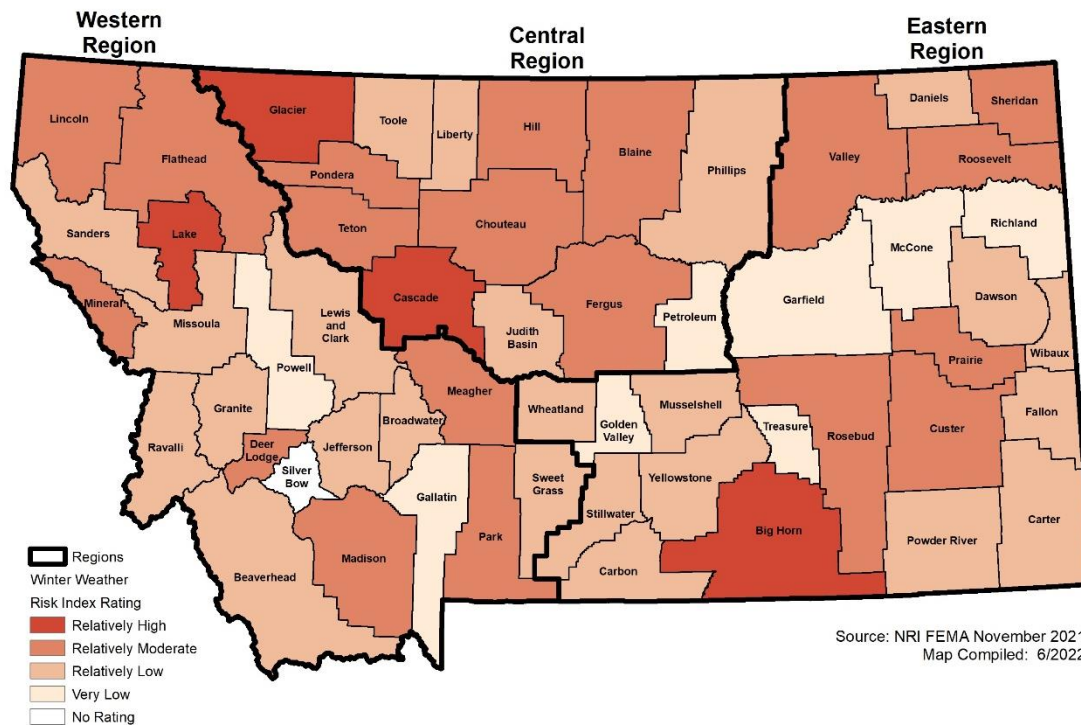
Figure 4-60 NRI Risk Index Rating for Winter Weather
