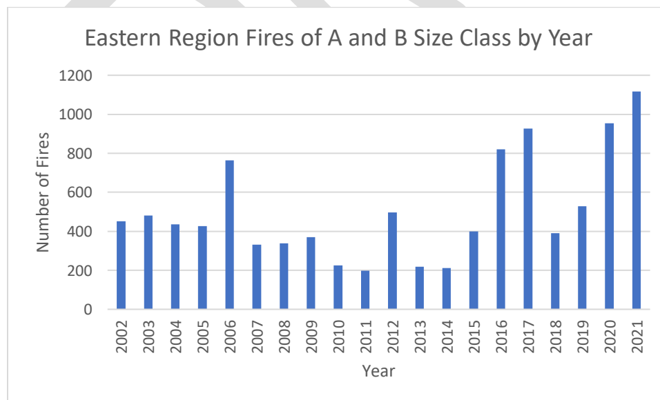
Figure 4-87 Number of Wildfire in Eastern Montana Region by Year and Size Class A-B, 2002 to 2021
