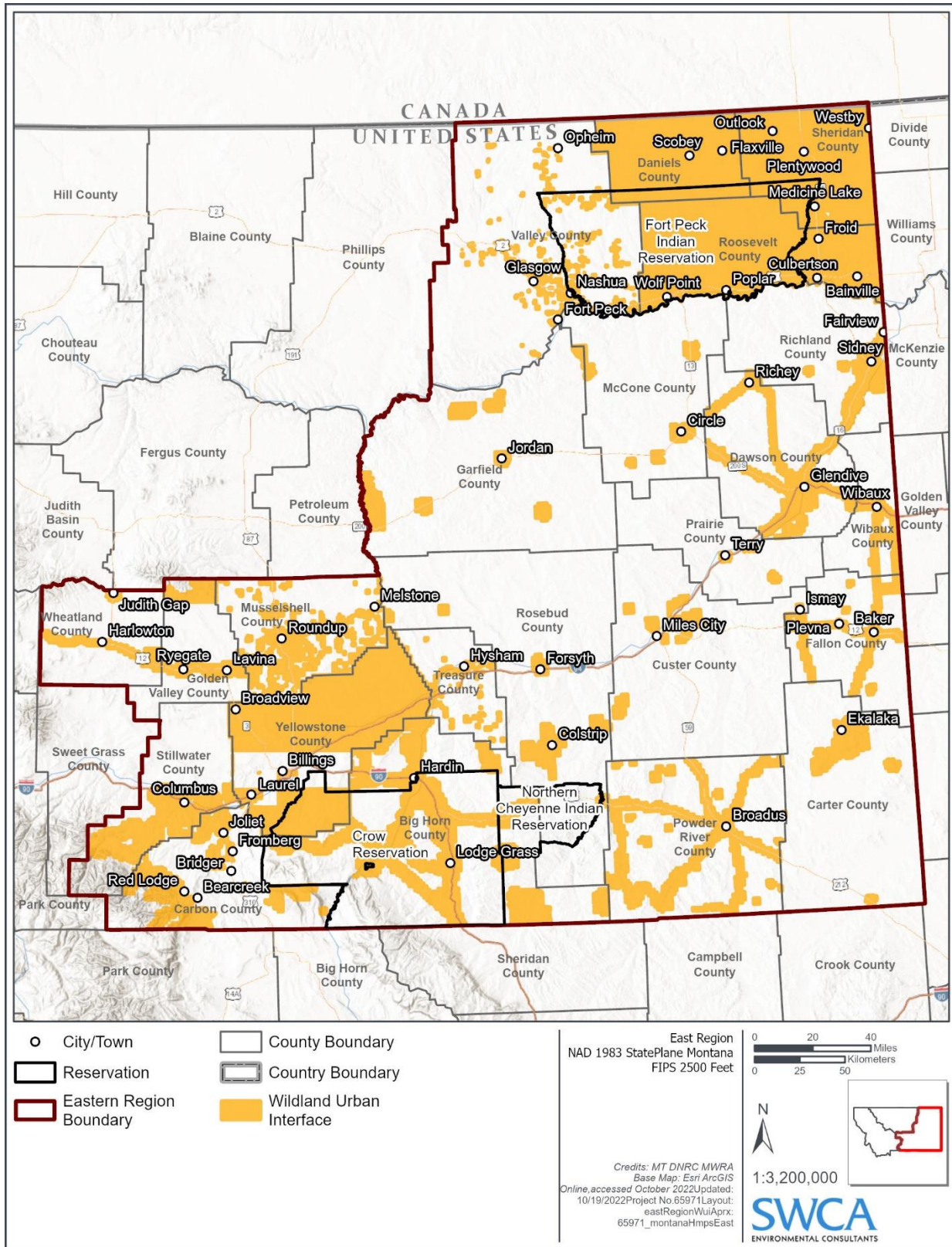
Figure 4-86 Wildland Urban Interface Delineation
