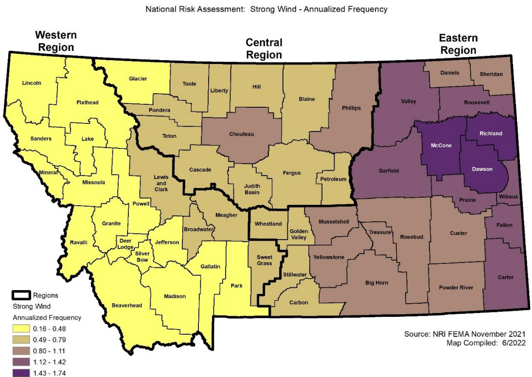
Figure 4-73 Annualized Frequency of Strong Wind Events by County
