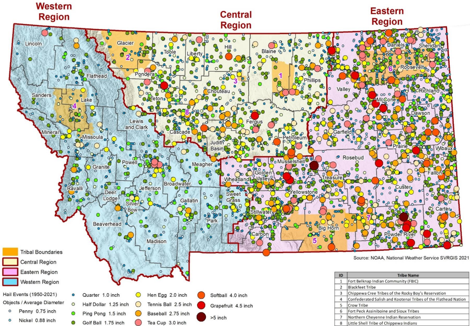
Figure 4-44 Hail Events in Montana by Region (1955-2021)
