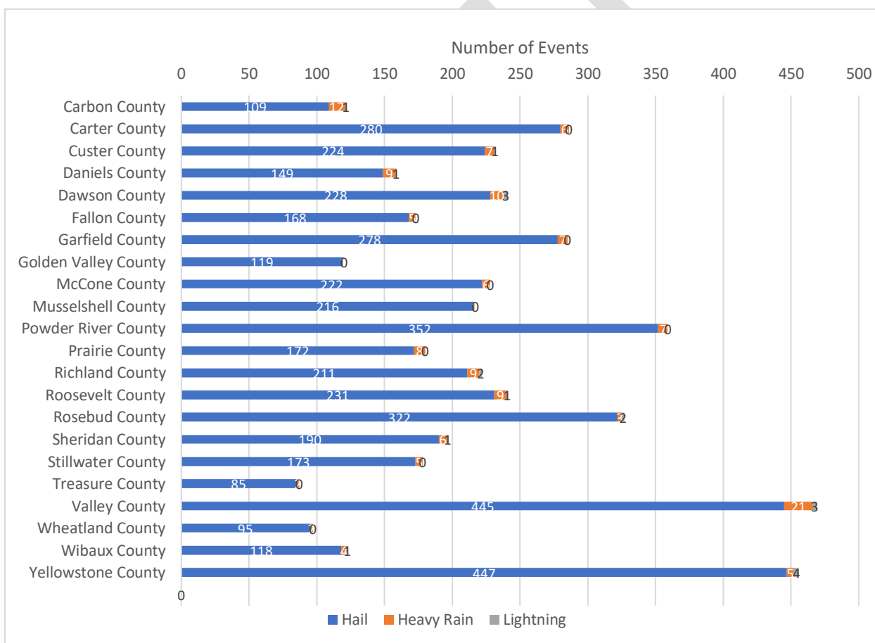
Figure 4-45 Summary of Severe Summer Weather Events by County in the Eastern Region
