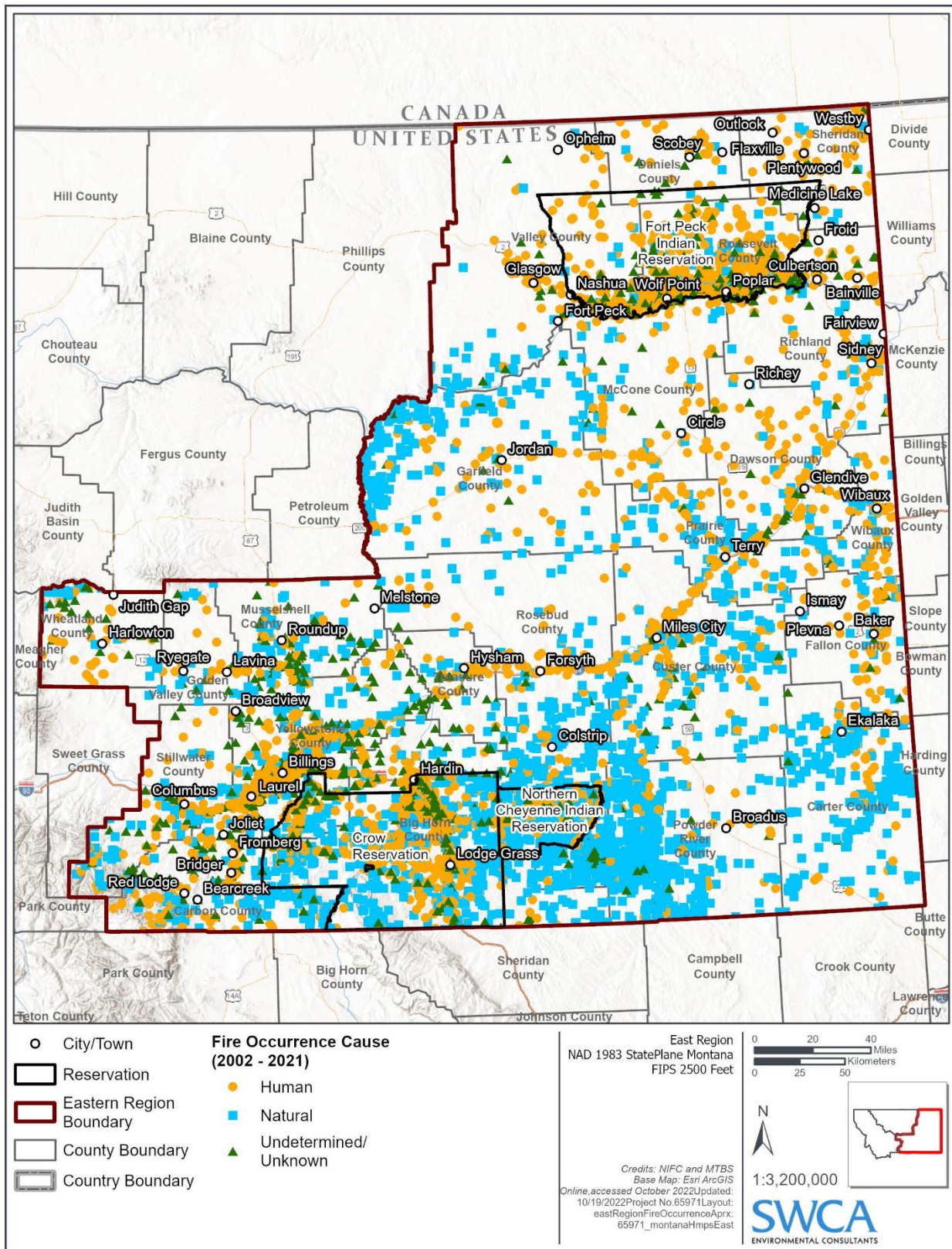
Figure 4-91 Fire Occurrence History in Eastern Montana, 2002 to 2021
