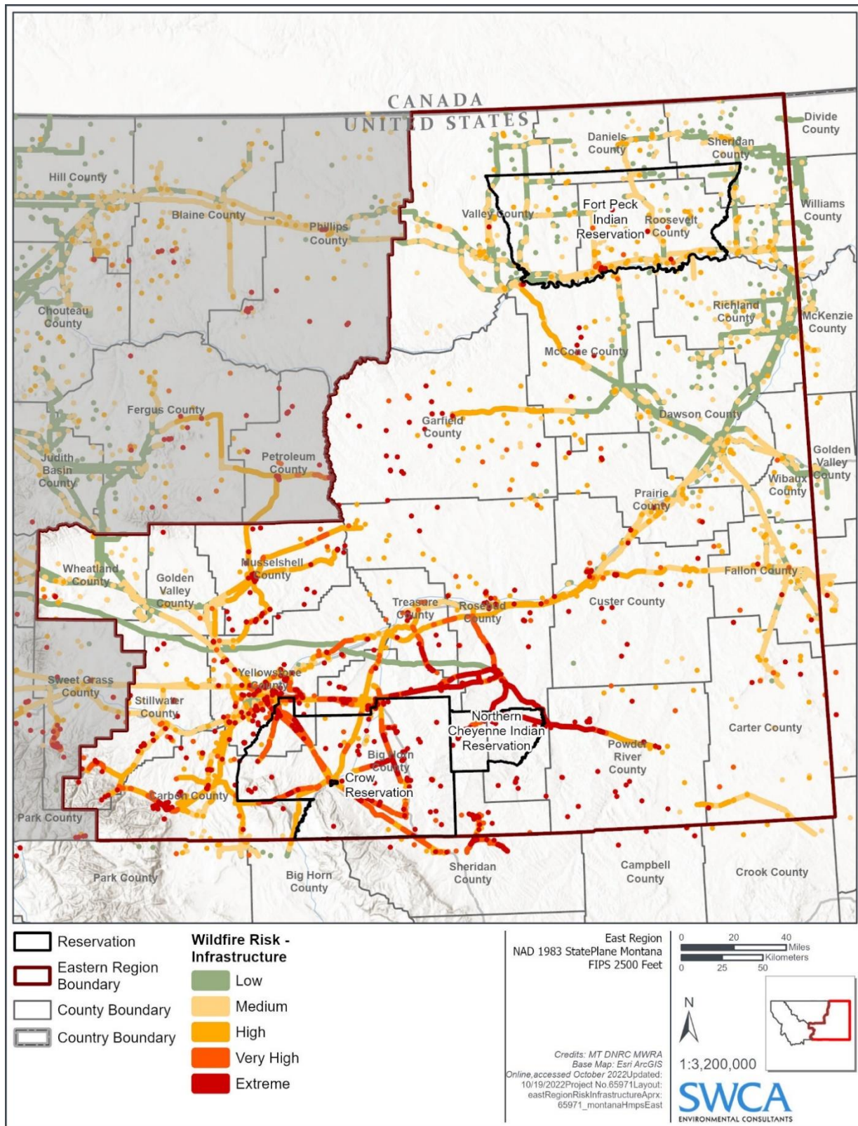
Figure 4-102 Wildfire Risk to Infrastructure in the Eastern Region
