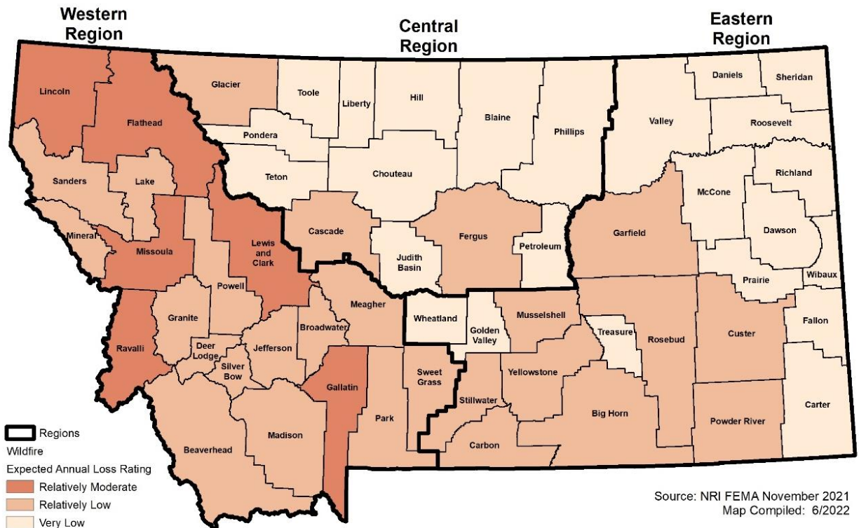
Figure 4-103 NRI Wildfire Expected Annual Loss Rating by County
