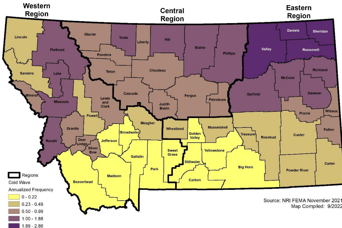
Figure 4-55 NRI Annualized Frequency of Cold Events by County
