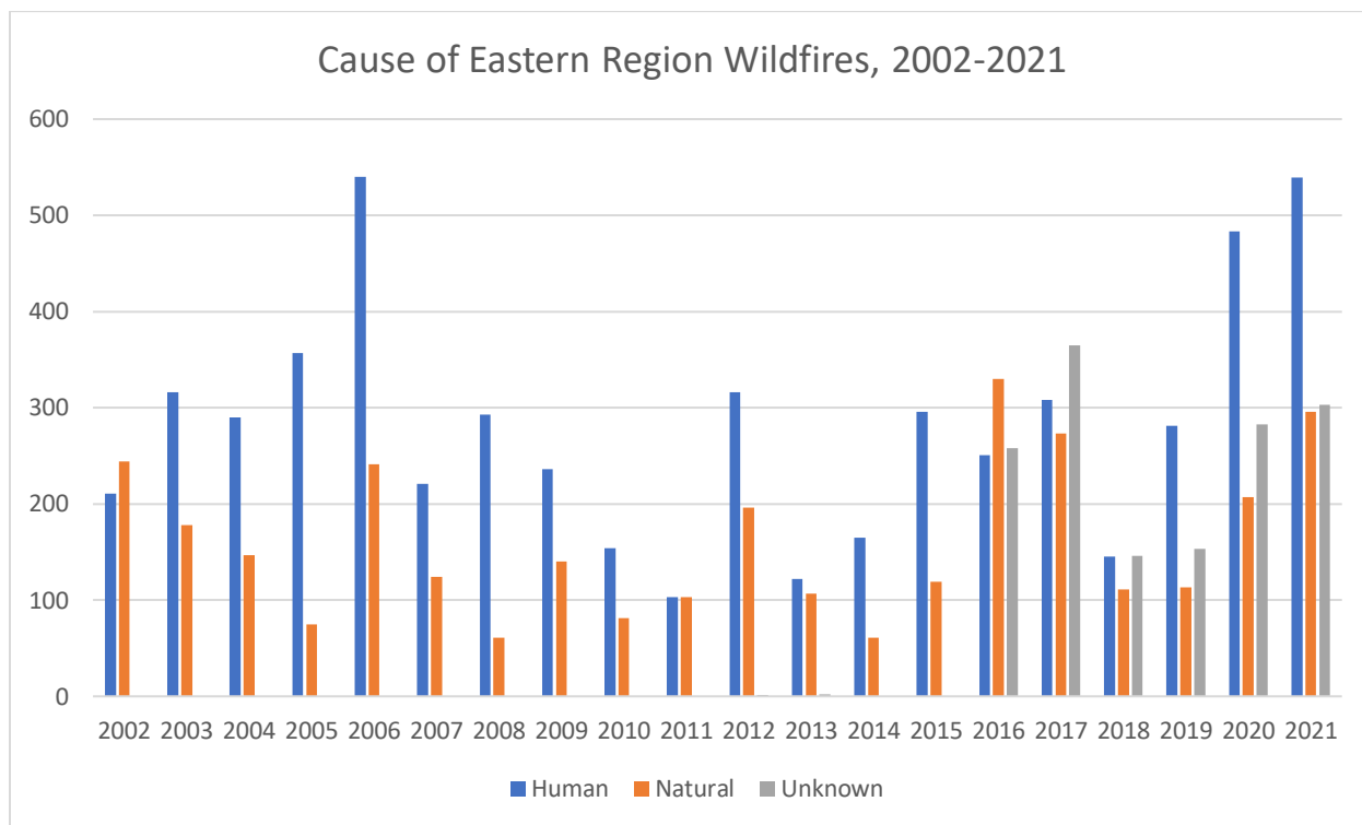
Figure 4-89 Number of Wildfires by Cause, 2002 to 2021
