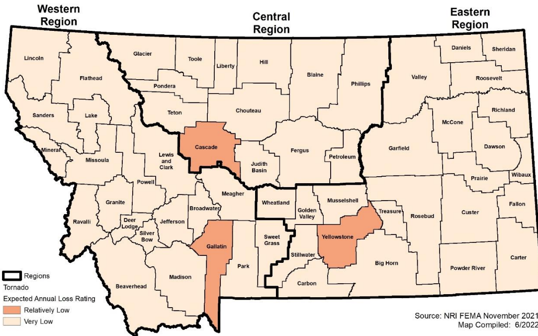
Figure 4-77 NRI Tornado Events Expected Annual Loss Rating
