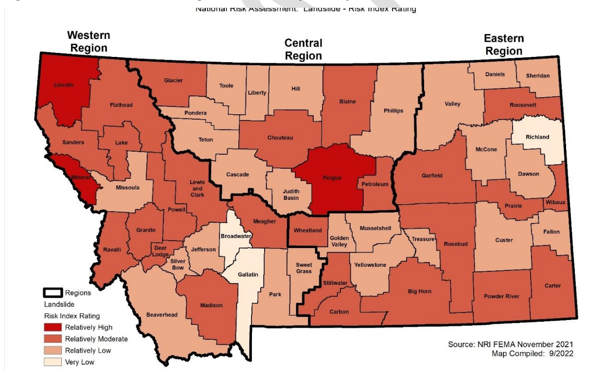
Figure 4-42 Risk Index Rating for Landslide by County
