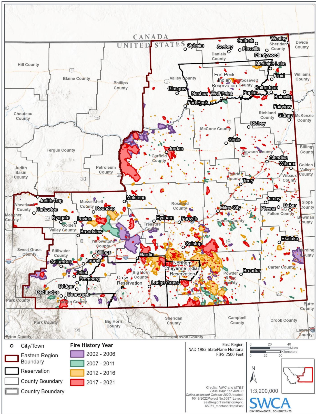
Figure 4-92 Fire History of Eastern Montana, Fire Perimeters, 2002-2021
