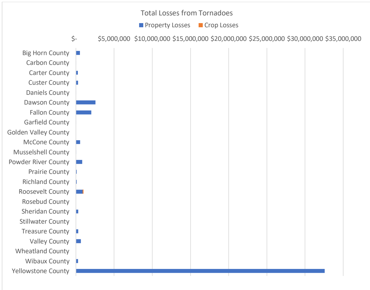
Figure 4-71 Total Losses from Tornadoes by County
