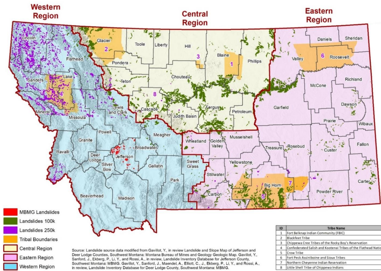
Figure 4-40 Montana Hazard Mitigation Planning Region Landslides
