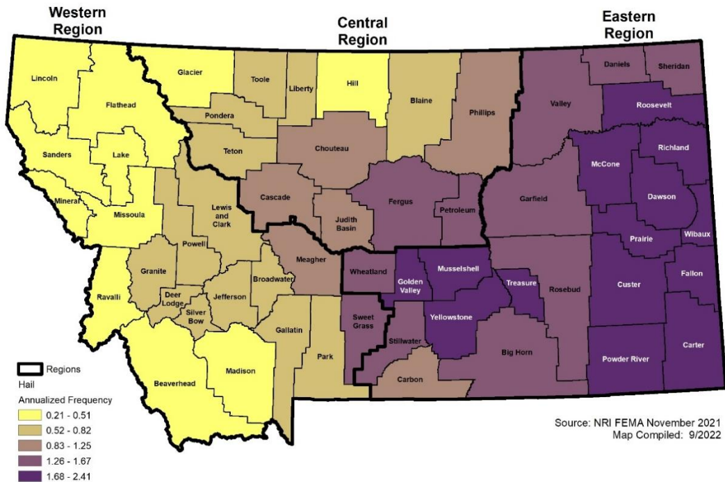
Figure 4-48 NRI Annualized Frequency of Hail Events by County
