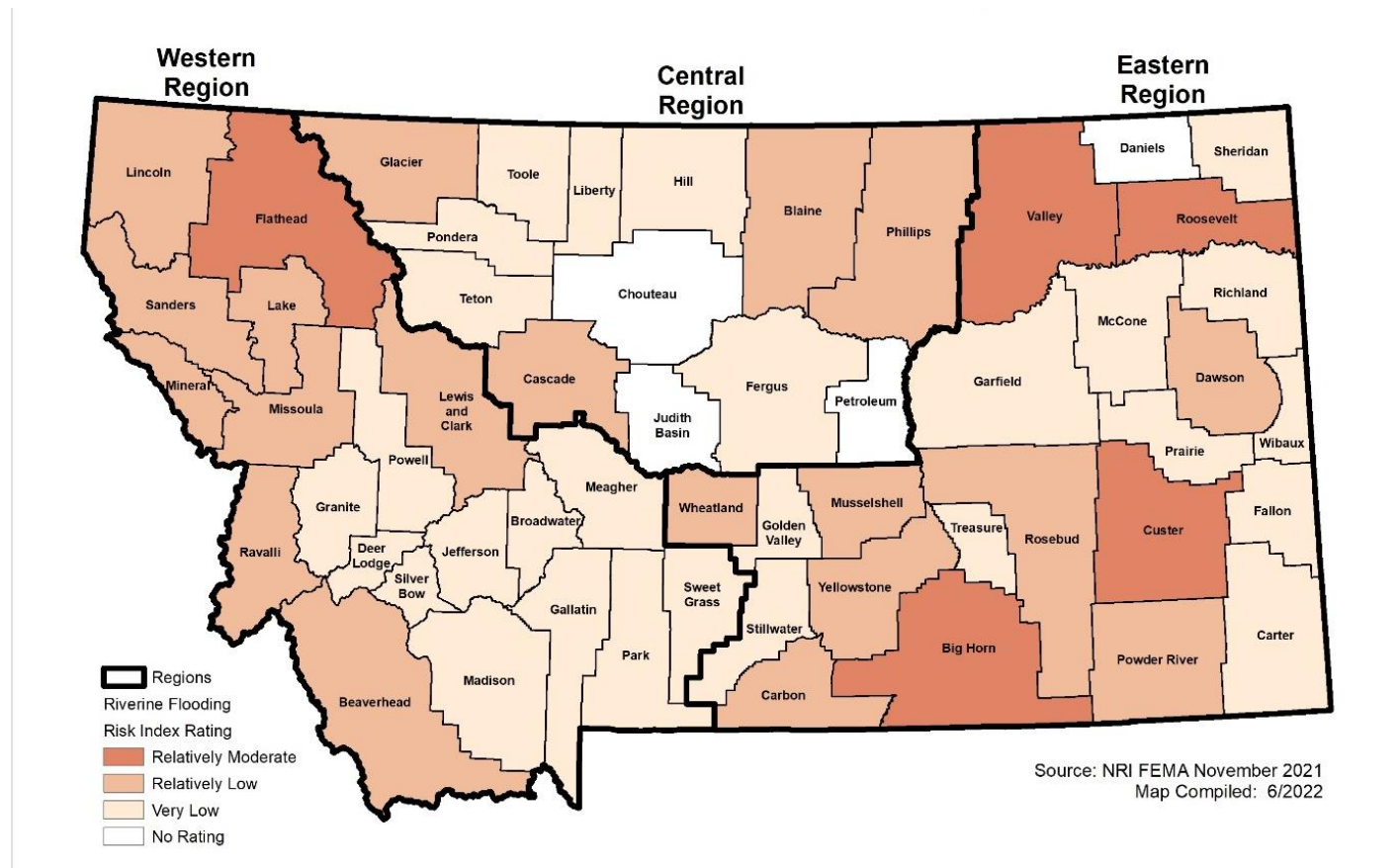
Figure 4-30 Risk Index Rating for Riverine Flooding by County
