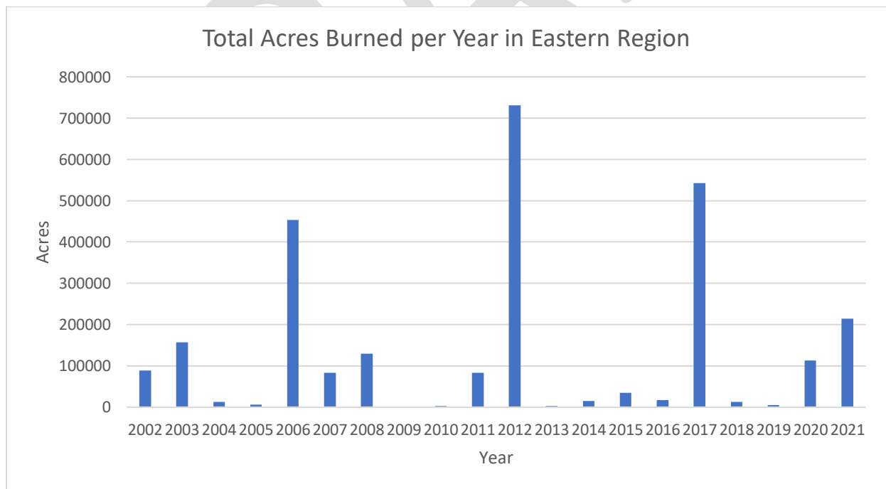
Figure 4-90 Total Acres of Burned per Year in Eastern Region, 2002 to 2021
