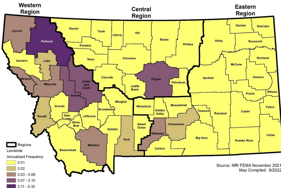
Figure 4-41 NRI Annualized Landslide Frequency Montana Eastern Region
