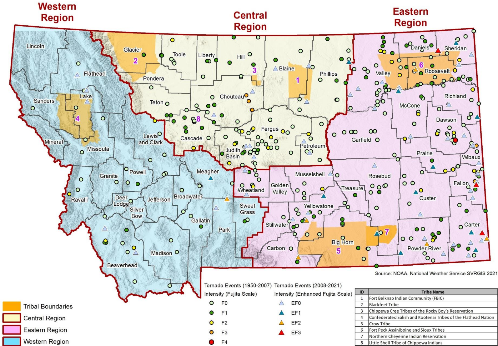
Figure 4-68 Past Tornado Events in Montana by Region (1950-2021)
