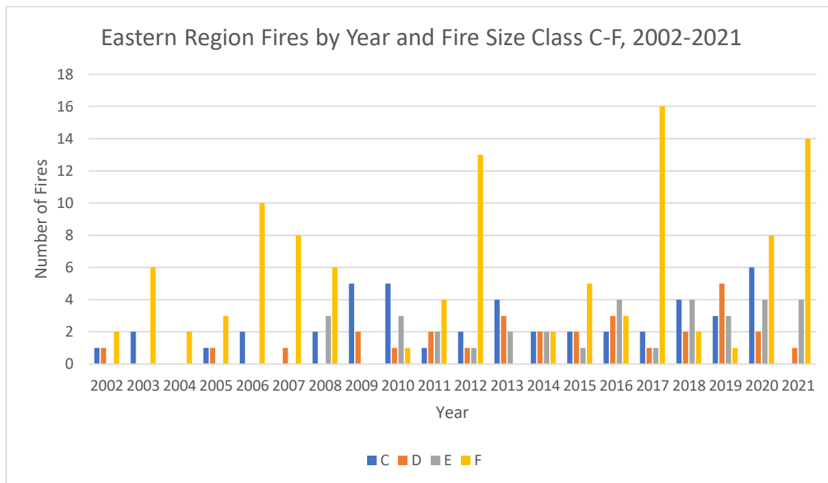
Figure 4-88 Number of Wildfire in Eastern Montana Region by Year and Size Class C-F, 2002 to 2021
